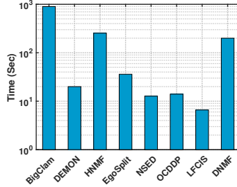
Fig. 6: Running time comparison.
