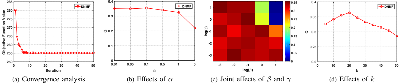
Fig. 4: Convergence and parameters sensitivity analyses of DNMF.
