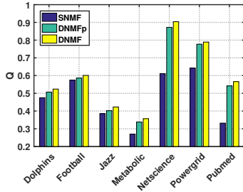
Fig. 5: Ablation study.
