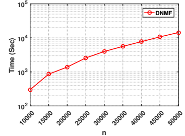
Fig. 7: Scalability testing.
